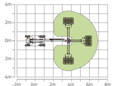
Range of Jib Swing Motion ZA10RJE
